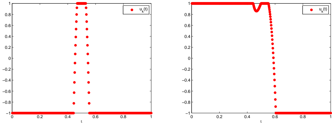
Figure 4.3: Approximate optimal controls after 1000 iterations when \theta = 2 (left) and \theta = 3 (right) for Example 4.3 with N = 500 .
