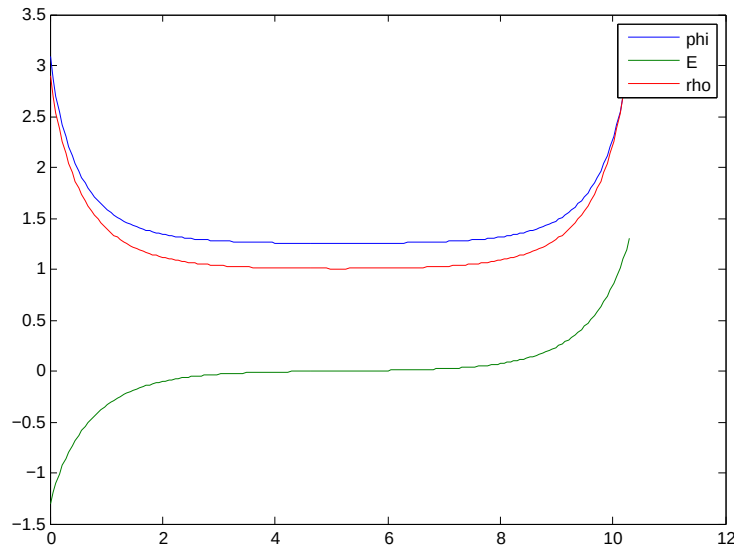
Figure 6.2: Example 6.2: The solution for the subsonic case.
