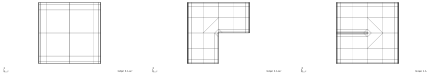
Fig. 4 Examples of geometric boundary layer meshes generated by Netgen/NGSolve [34] that are used for the three domains \Omega = \Omega_j , j = 1, 2, 3 , ordered from left to right.
