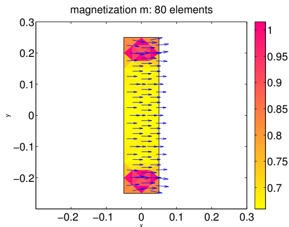
FIGURE 2. Magnetization m_N .
