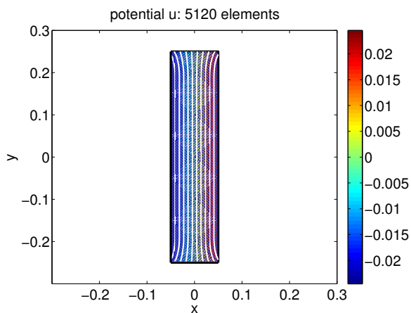
FIGURE 1. Potential u_N .
