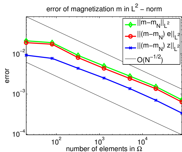
FIGURE 4. Convergence of m .
