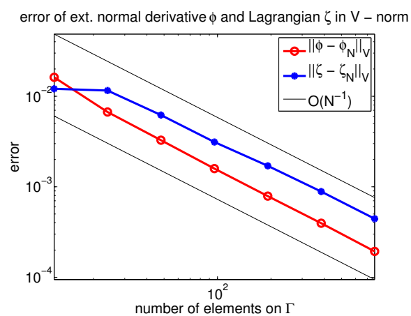
FIGURE 6. Convergence of \phi and \zeta .
