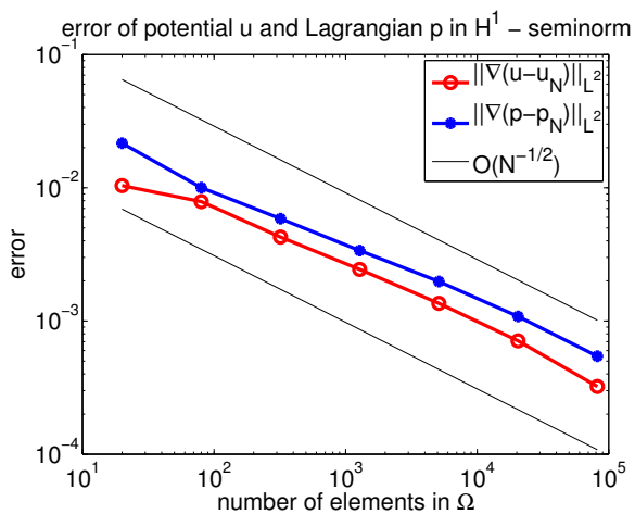
FIGURE 5. Convergence of u and p .
