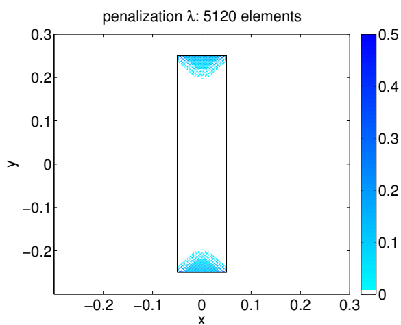
FIGURE 3. Penalization \lambda_N .
