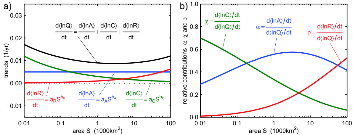
Figure 1. Schematic of a hypothetical mixing model and scaling behavior of flood trends (equations (1) and (3)): (a) flood trends (d\langle \ln Q \rangle / dt) and trend components (d\langle \ln A \rangle / dt, d\langle \ln C \rangle / dt) and (d\langle \ln R \rangle / dt) as a function of catchment area S ; (b) relative contributions of the atmosphere ( \alpha ), catchment ( \chi ), and river ( \rho ) components of flood peak trends as a function of catchment area S . The colorcode for this and all following figures: blue = atmosphere, green = catchment, and red = river.
