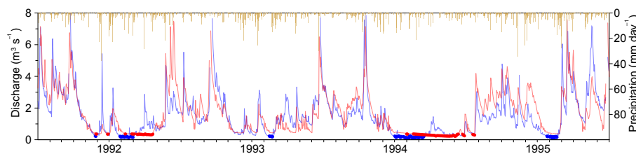
Figure 5. Comparison of observed (blue) and simulated (red) flow for Hoheneich/Braunaubach, 291.5 km 2 ). Thick lines show flows below low-flow quantile Q_{95} . Model simulations are based on calibration variant w_Q = 0.5 in the period 1998–2008. The relative difference between Q_{95} estimated from simulated and observed flows is 8 %.
