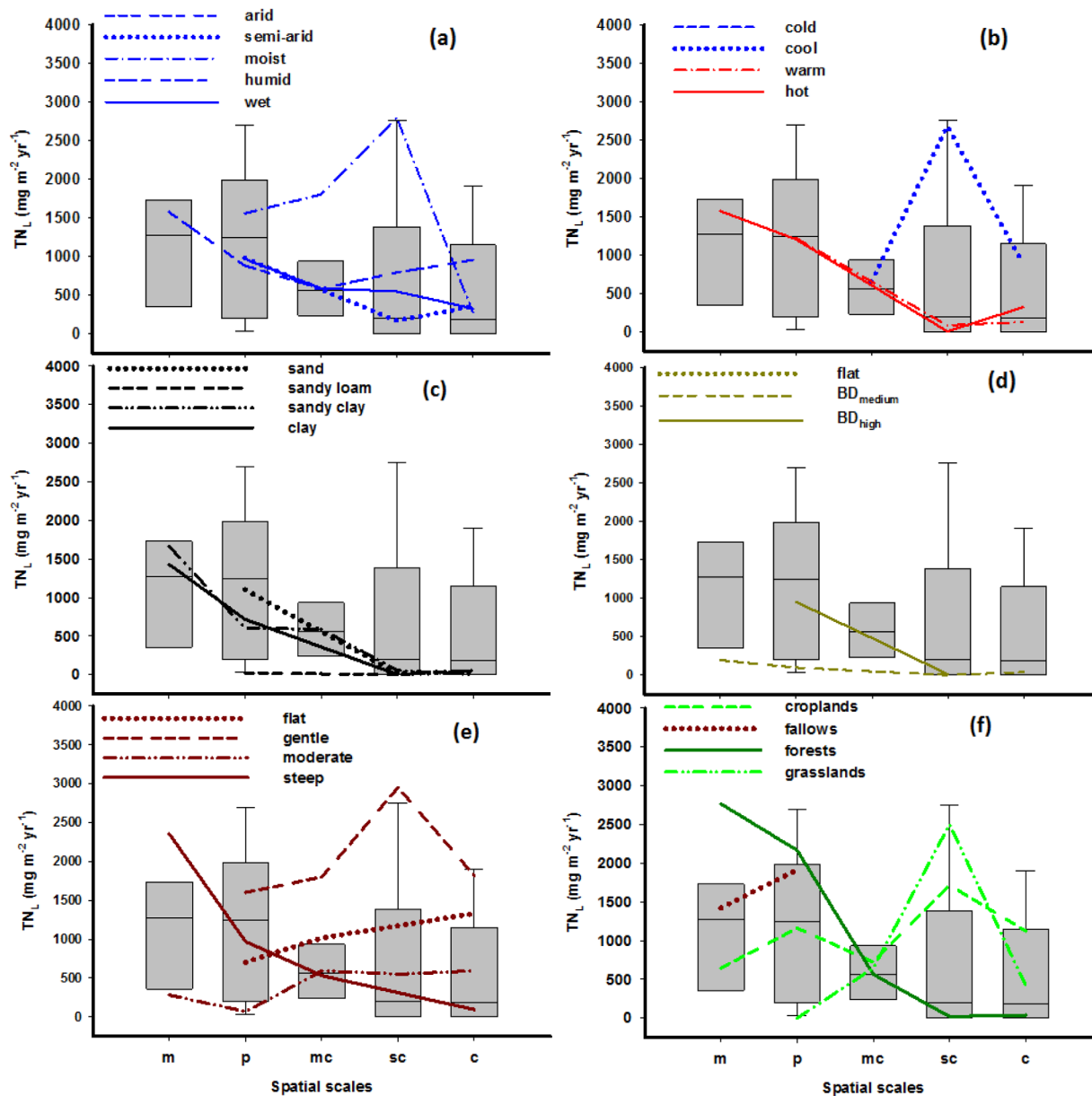
Figure 7. Total nitrogen losses (TN L ) from the literature for each of the spatial scales (box plots), and stratified by (a) mean annual precipitation, MAP, (b) mean annual temperature, MAT, (c) clay content, CLAY, (d) soil bulk density, BD, (e) slope gradient, S, and (f) land use LU (lines). The spatial scales are m: microplot, p: plot, mc: microcatchment, sc: subcatchment, and c: catchment. For classifications, see Table 7. Each box plot shows the median line, 25–75% range, and lower and upper limit of the nonoutlier range.
