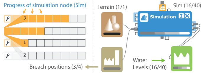
Fig. 8. Progress visualization with World Lines (WL) vs. inside the flow diagram. WL comprise 4 tracks for 4 different breach positions. WL show progress on a per-frame level, the flow diagram on a per-node level. The figure labels depict (calculated frames/frames to calculate).
