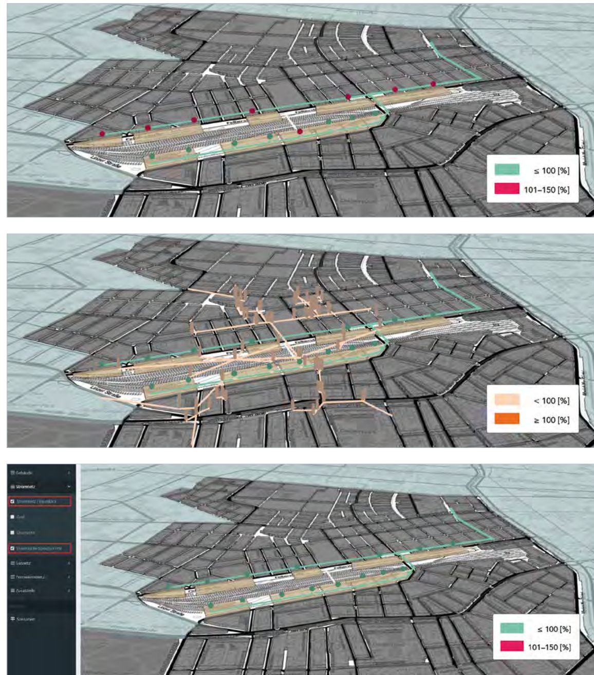
▲ Figure 56 Utilisation rate in the electricity grid for stations and lines at block level (top), utilisation rate in the electricity grid for stations and lines in combination with the heat supply for the district provided by district heating at block level (middle) and utilisation rate in the electricity grid for stations and lines in combination with PV systems and accumulators at block level (bottom). © URBEM/TU Wien
