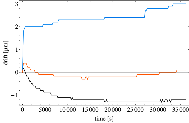
Figure 3.39: Drift measurement of the system loaded with 3.95 kg, which has been unstressed before. The three lines correspond to the three linear gages used.
