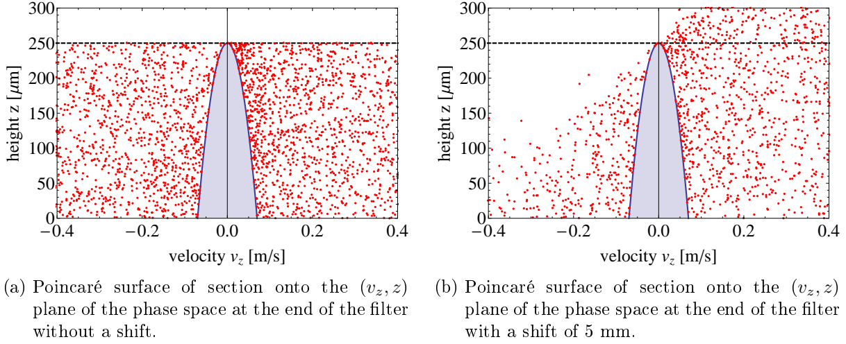
Figure 2.6: Comparison of the phase space at the end of the vectorial velocity filter with and without a shift of the selector's scatterer versus its lower mirror, obtained from three-dimensional Monte Carlo simulations.
