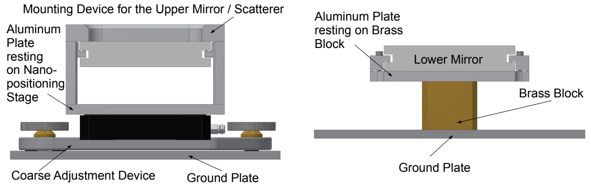
(a) Only parts responsible to hold the upper mirror / scatterer are shown. (b) Only parts where the lower mirror rests on are shown.
