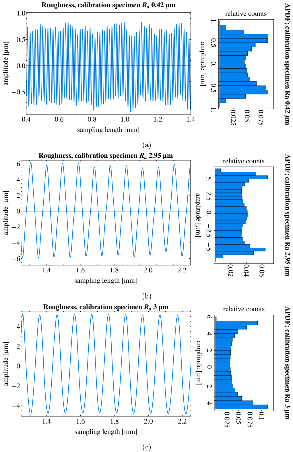
Figure 3.22: Filtered roughness profiles and APDF of (a) calibration specimen R_a = 0.42\mu\text{m} , (b) calibration specimen R_a = 2.95\mu\text{m} , (c) calibration specimen R_a = 3\mu\text{m} ; only 1mm of the measured length is shown to increase visibility; information of full measured length taken for the APDFs
