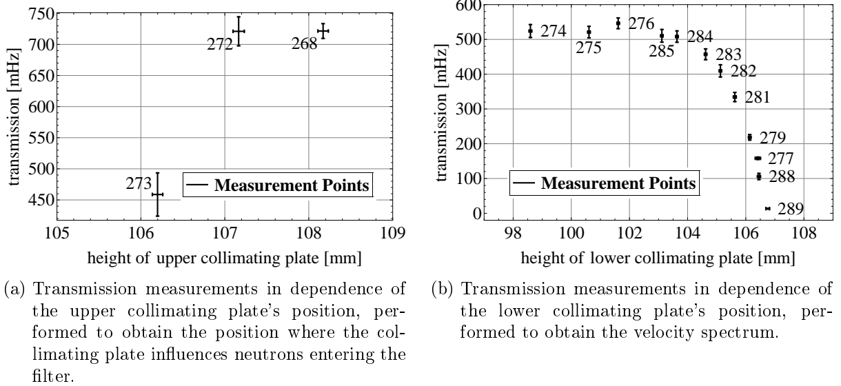
Figure 4.2: Transmission measurements in dependence of the collimating plates' position, performed to obtain the velocity spectrum.
