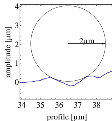
Figure 3.32: “Stylus tip” on surface measured using SEM
