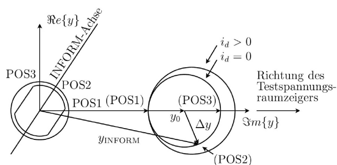
Determination of Rotorposition y_{\text{INFORM}}
