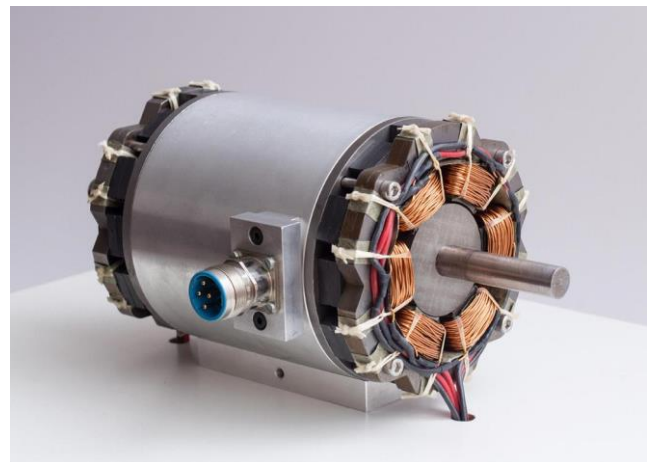
Sensorless magnetic bearings – e.g. for the rotor of an electric motor
