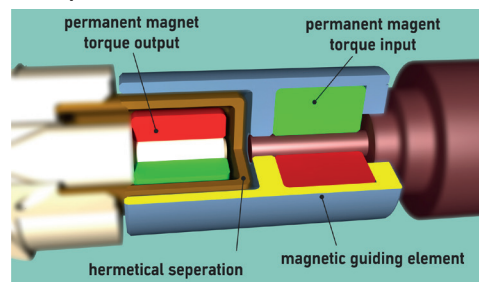
Fig 1: cross-sectional-view of the miniature magnetic coupling
