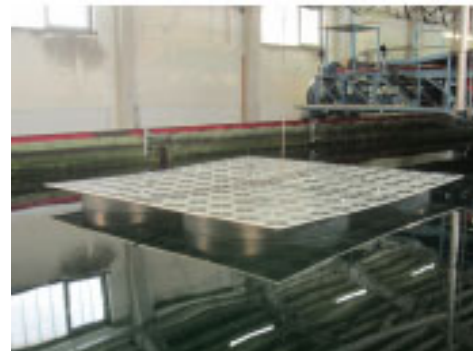
Fig. 1: HELIOFLOAT Platform 4m*4m model
